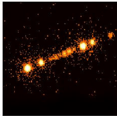
Chandra
