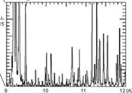
Chandra Grating
