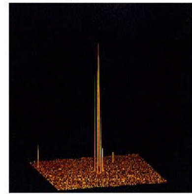
Chandra
