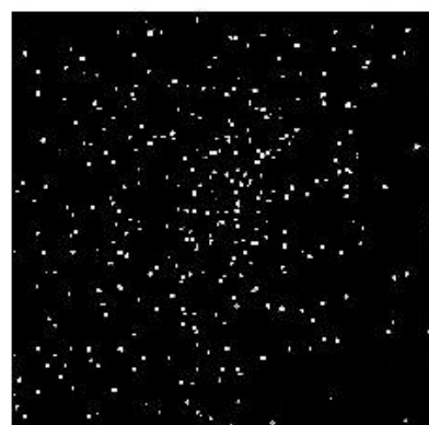
Chandra
