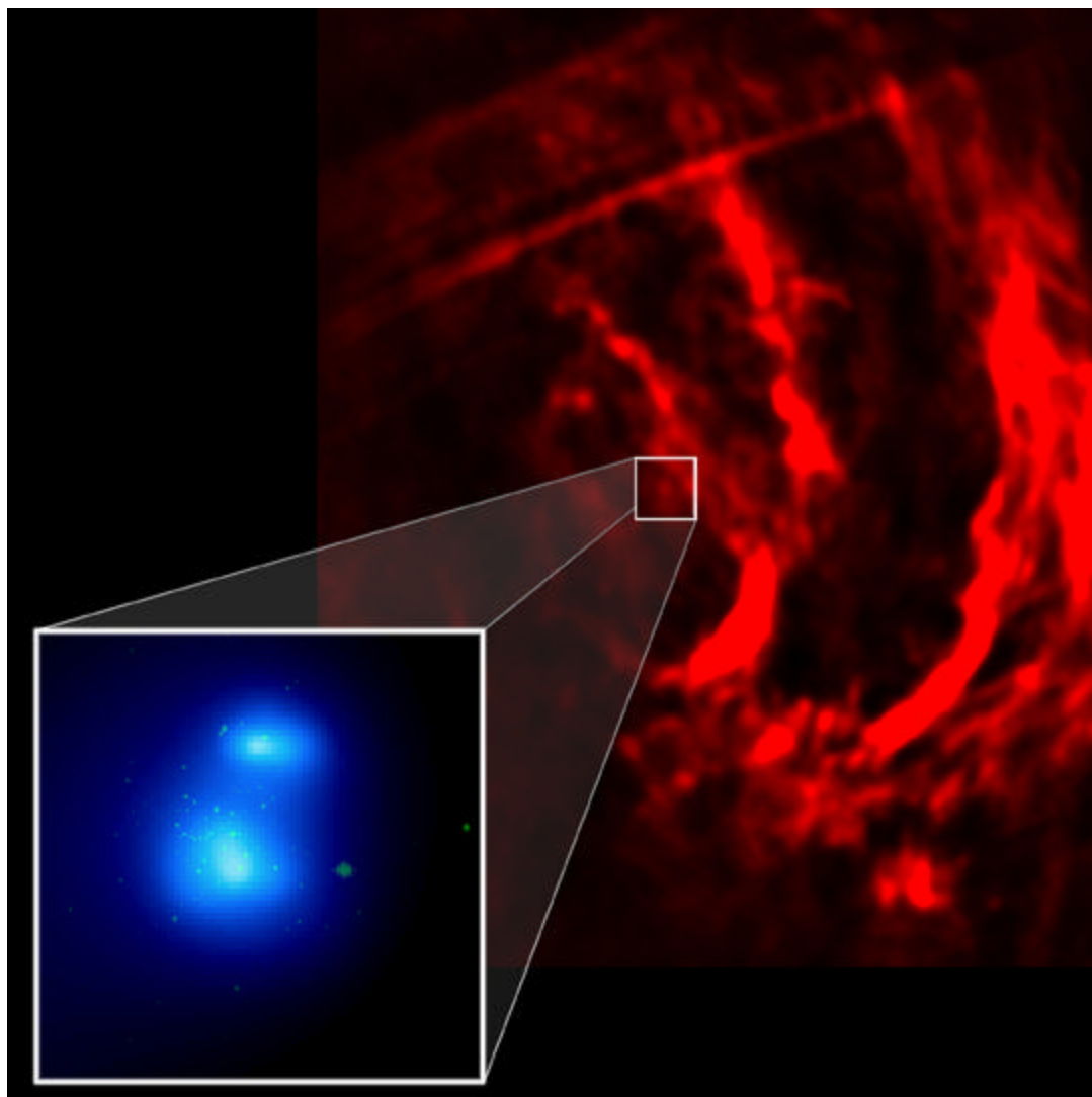
X-ray/Infrared/Radio Composite
