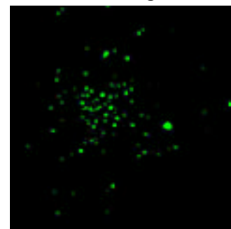
Infrared
